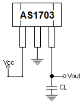
Figure 1, Typical Application Circuit of AS1703
