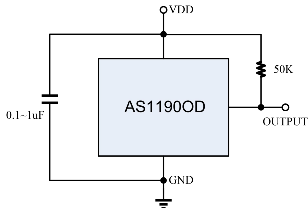
Figure 1, Typical Application Circuit of AS1190OD
